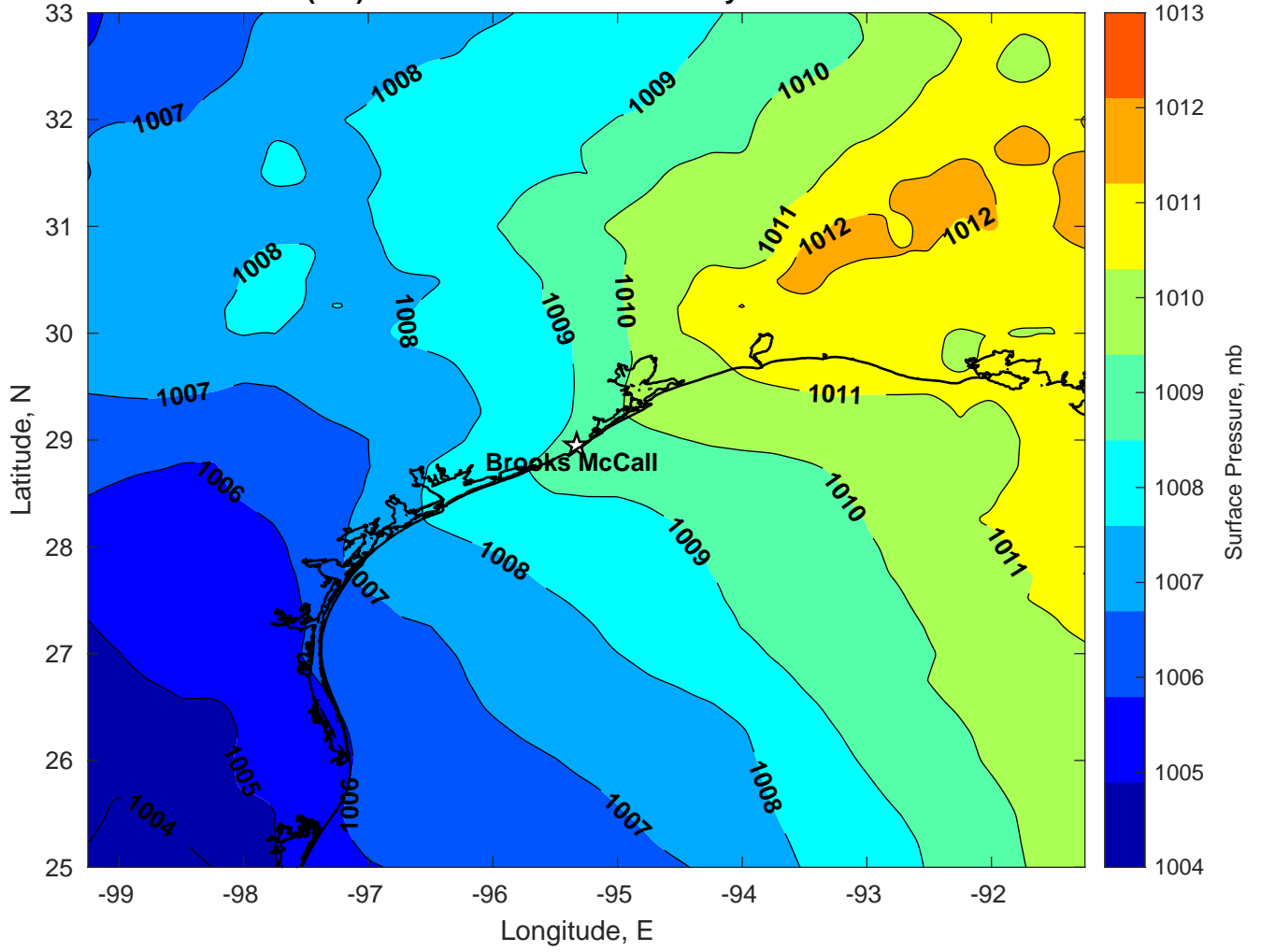
Surface Pressure (mb) for Brooks McCall at 02-May-2024 18:00:00
